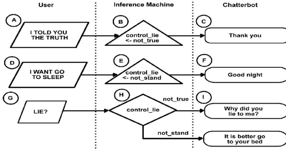
Figure 3.Flowchart of Ambiguity Treatment.
